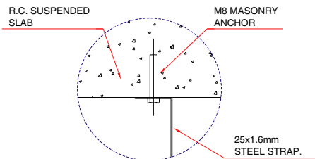
06 DETAIL D SCALE 1/5
