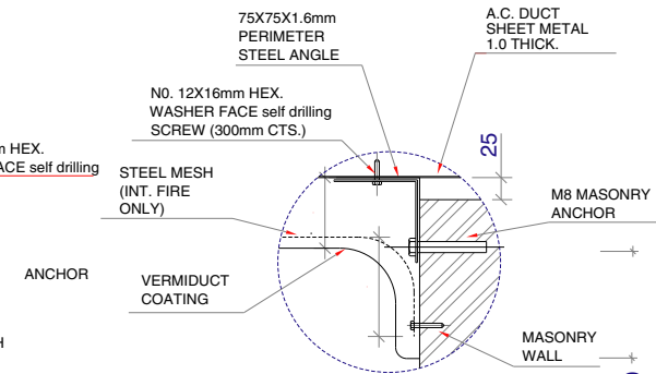
03 DETAIL A SCALE 1/5
