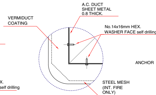
04 DETAIL B SCALE 1/5
