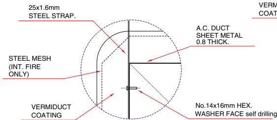
05 DETAIL C SCALE 1/5
