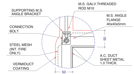
06 DETAIL D SCALE 1/5
