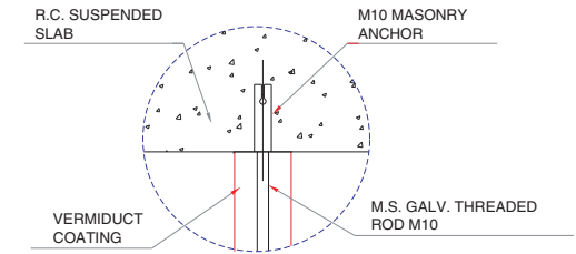
07 DETAIL E SCALE 1/5
