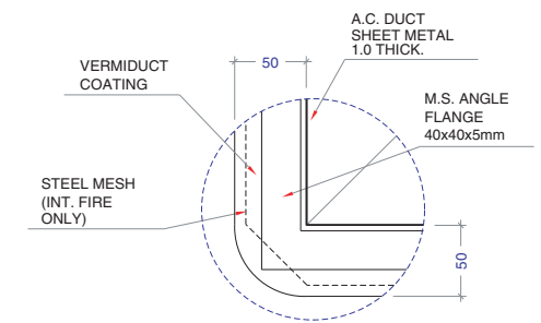
05 DETAIL C SCALE 1/5
