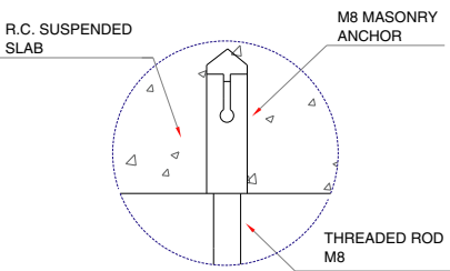
06 DETAIL D SCALE 1/5
