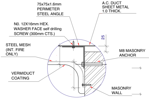
03 DETAIL A SCALE 1/5
