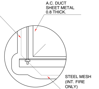
04 DETAIL B SCALE 1/5
